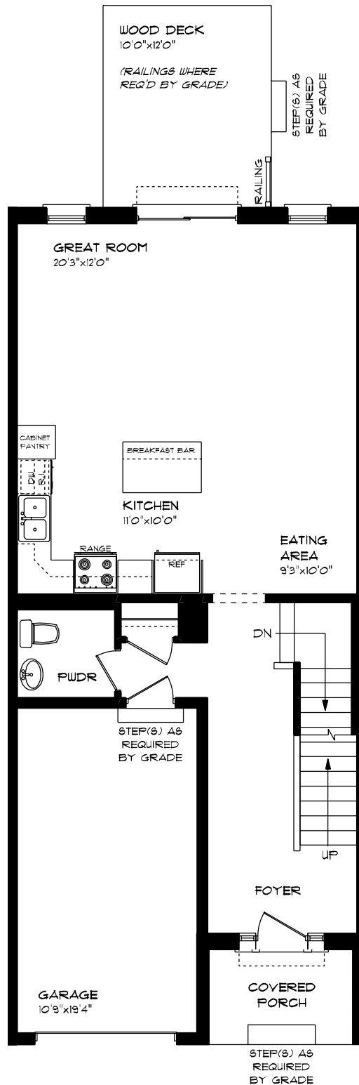
SHELTON (ESSENTIAL SPECS) LOT 6B (#113) WILLOW DRIVE MAIN FLOOR PLAN 9' MAIN FLOOR CEILING APPROX. 165 SQ. FT.
