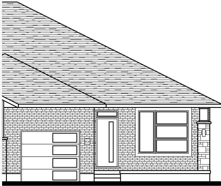
ARBOR (ESSENTIAL SPECS) LOT 42F (#16) FINCH STREET FRONT ELEVATION 9' MAIN FLOOR CEILING APPROX. 1,225 TOTAL SQ. FT.
